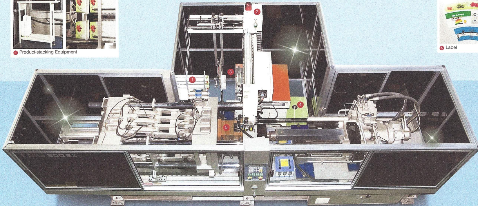
3 Label Feeder
